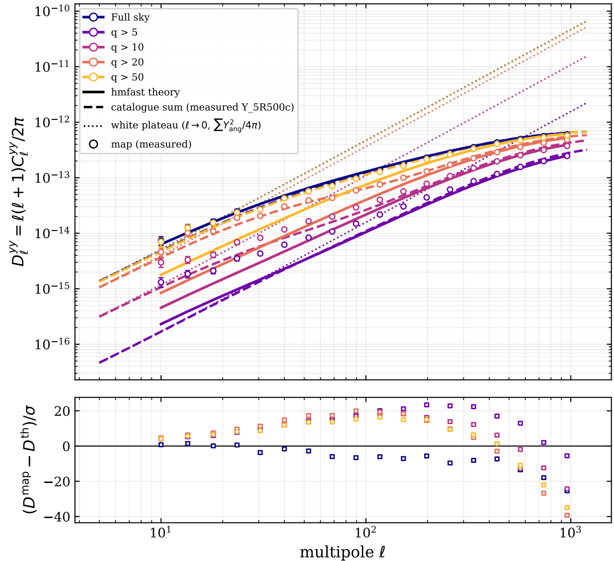
Unrotated z < 0.35 tSZ power spectrum: map vs hmfast ( B = 1.1093 , z_{\text{max}} = 0.35 )
