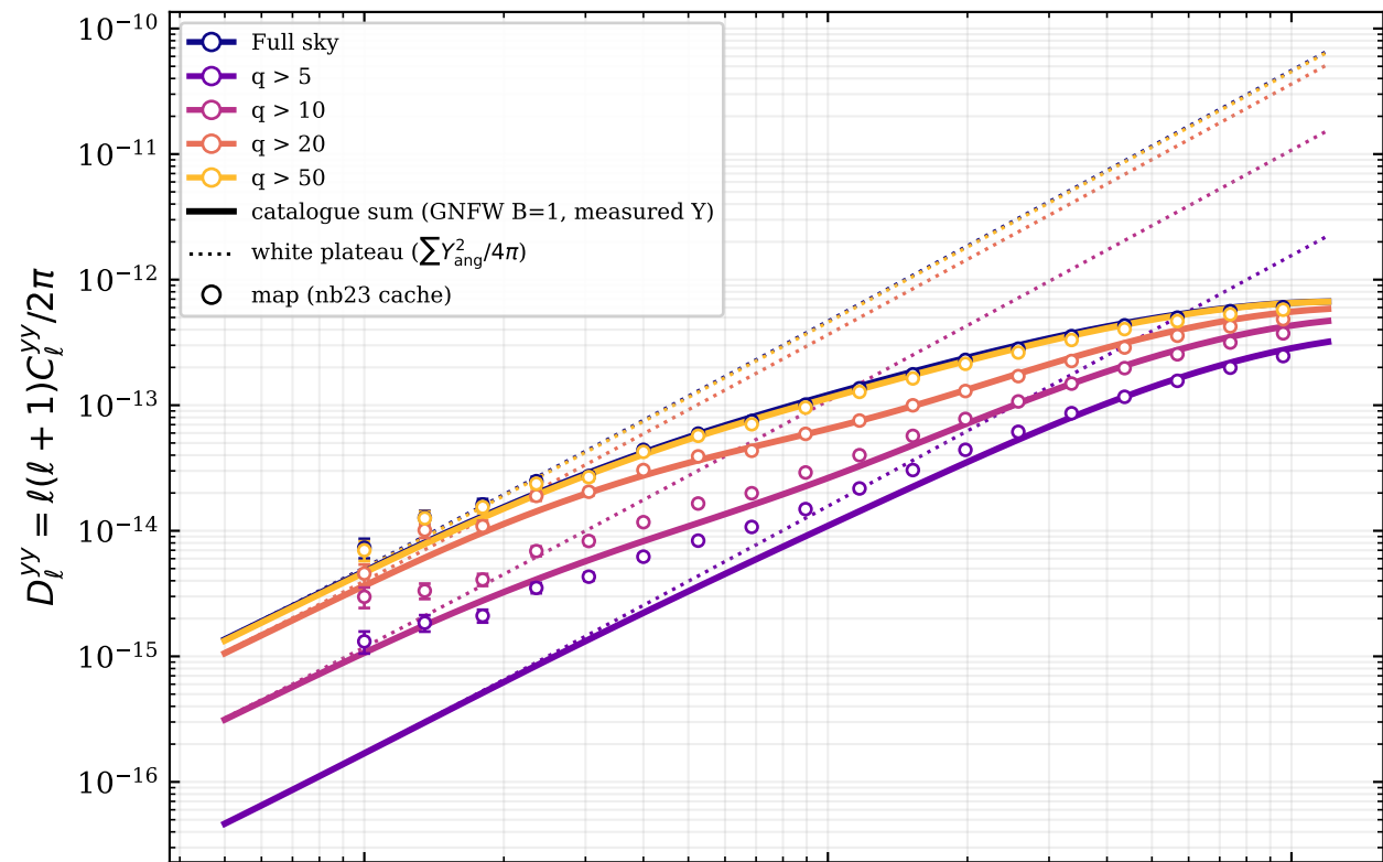
Unrotated z < 0.35 : map vs catalogue 1-halo sum (GNFW B = 1 , measured Y_{5R500c} )
