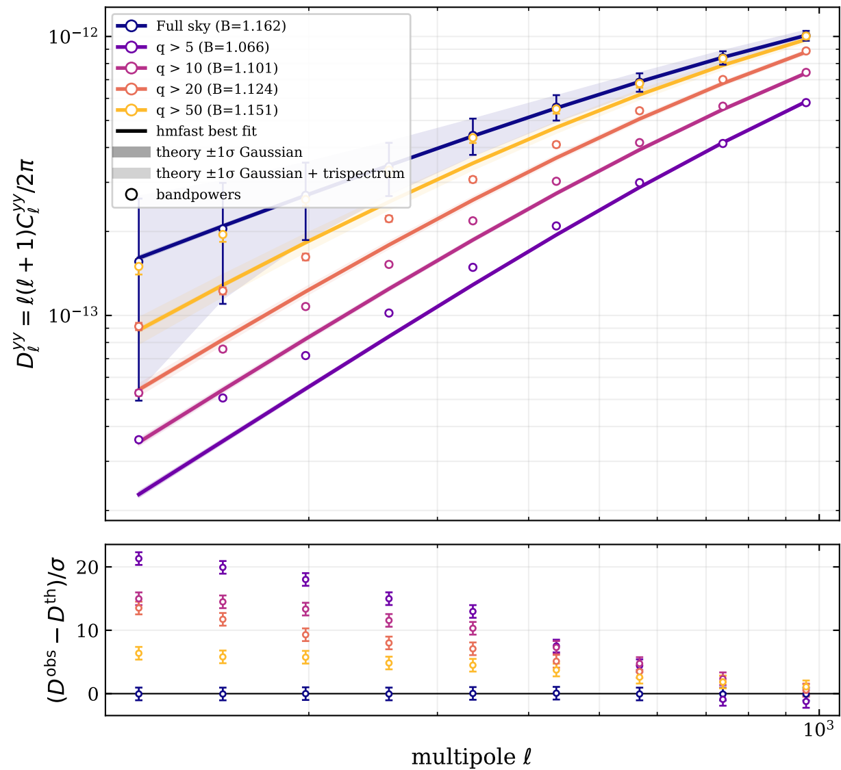
Best-fit tSZ PS (arnaudB1, \ell > 100 ; A10 GNFW, \sigma_{\ln Y} = 0.173 )
