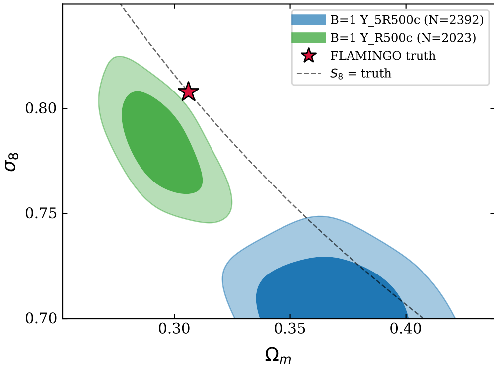
B=1: Y_{5R500c} vs Y_{R500c}
