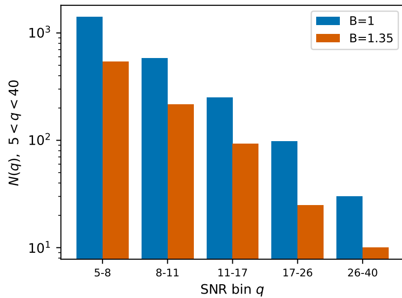
(b) SNR distribution
