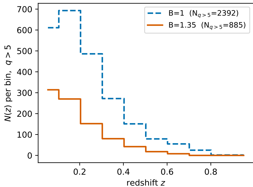
(a) Redshift distribution
