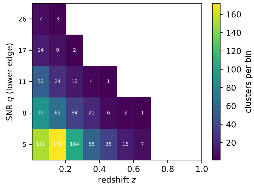
(c) N(z, q) , B=1.35
