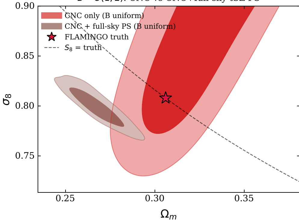
B \sim U(1, 2) : CNC vs CNC+full-sky tSZ PS
