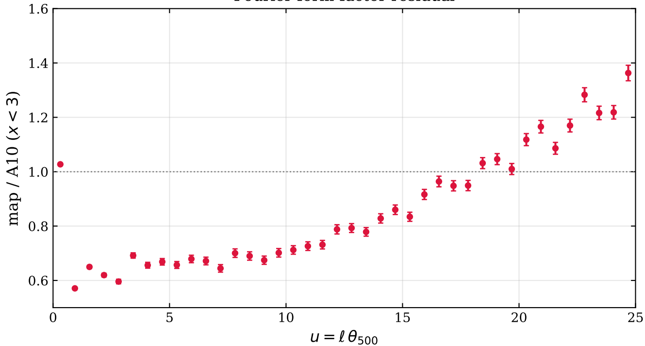
Fourier form-factor residual
