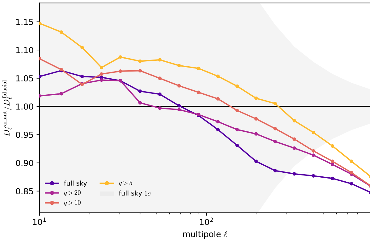
FLAMINGO L1_m9: f_{\text{gas}} - 8\sigma / fiducial ratio vs sky cut (18 Planck bins; empirical aperture q ; bands: full sky theory 1\sigma about 1)
