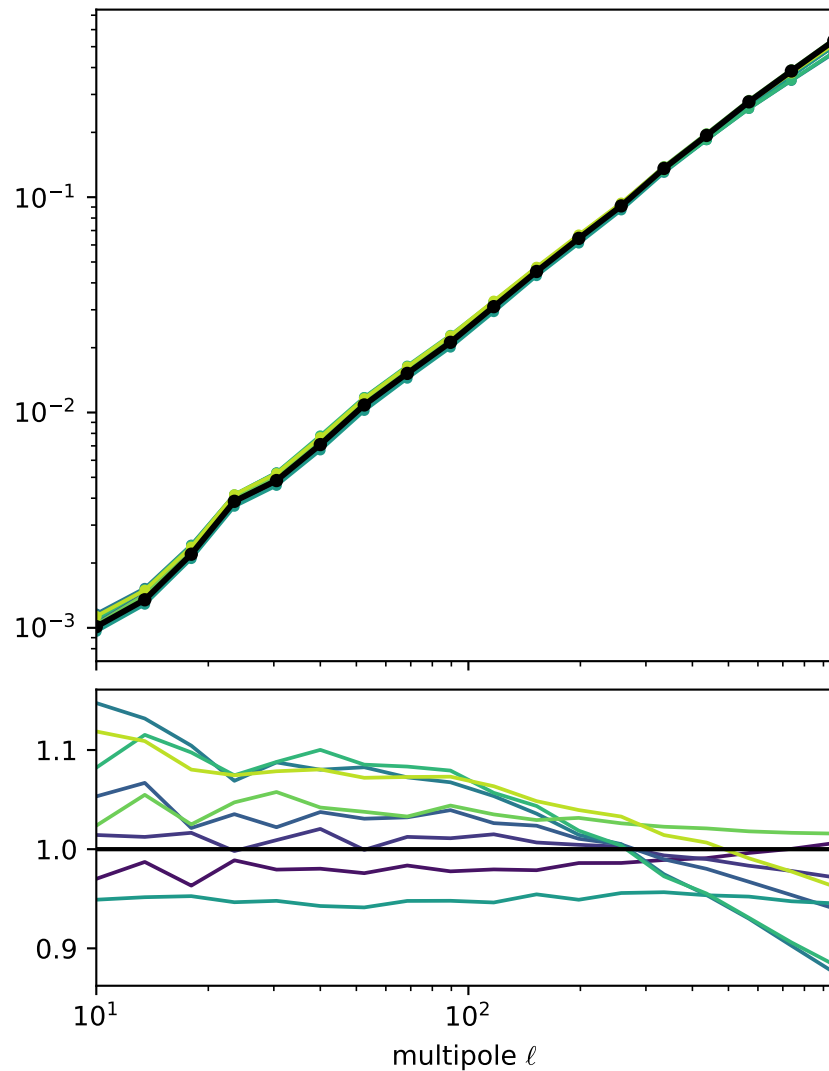
masked, q > 5
