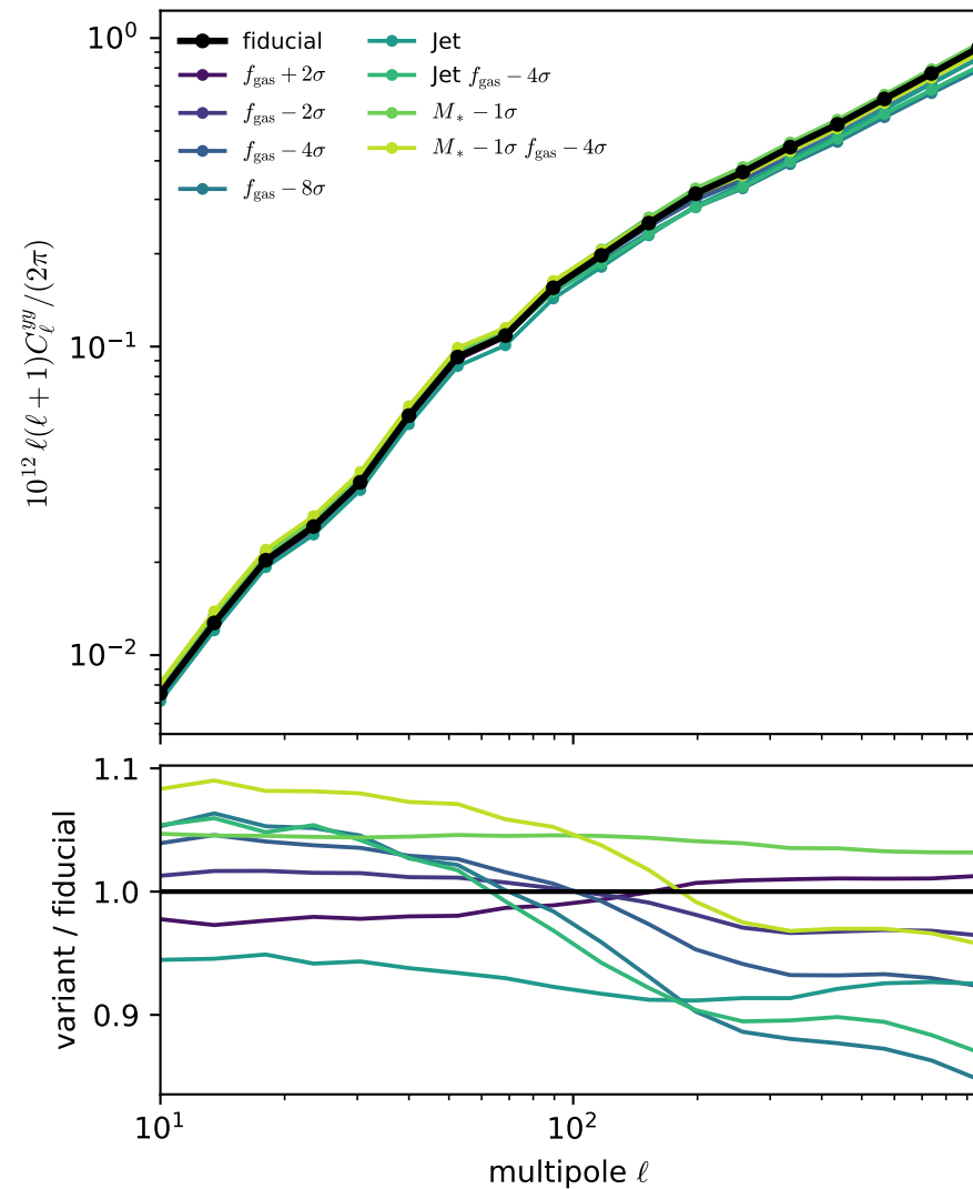
full sky
