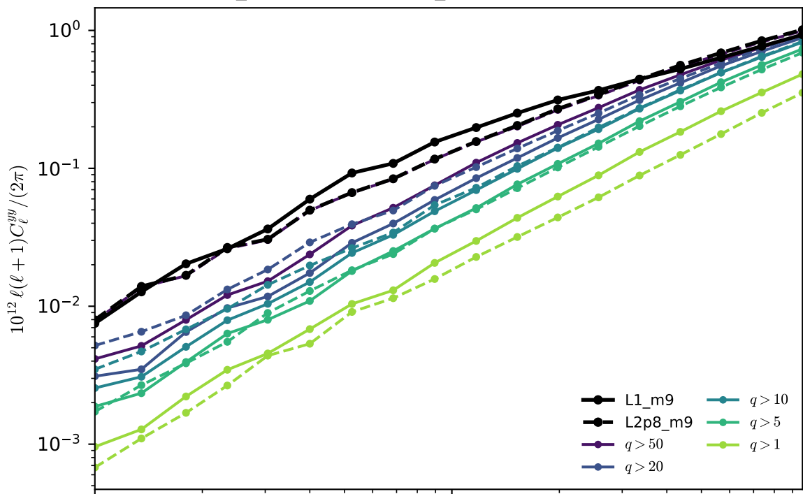
FLAMINGO masked tSZ: L1_m9 (solid) vs L2p8_m9 (dashed), 18 Planck bins, \alpha_{SZ} = 1.12 best-fit q
