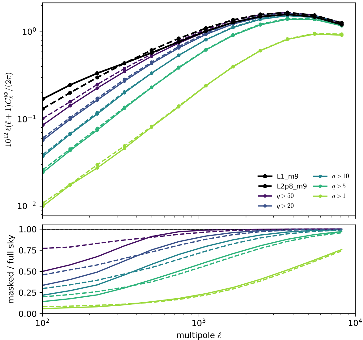
FLAMINGO masked tSZ: L1_m9 (solid) vs L2p8_m9 (dashed), \Delta \ln \ell = 0.4 log bins, empirical aperture q
