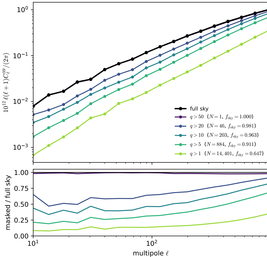
FLAMINGO L2p8_m9 fiducial (lc0): masked tSZ power spectrum ( \alpha_{\text{SZ}} = 1.12 best-fit q , 18 Planck bins)
