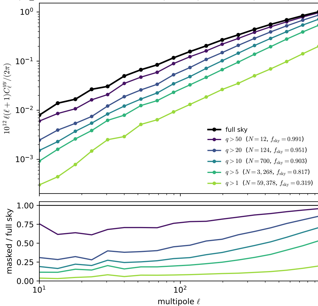
FLAMINGO L2p8_m9 fiducial (lc0): masked tSZ power spectrum (empirical aperture q , 18 Planck bins)
