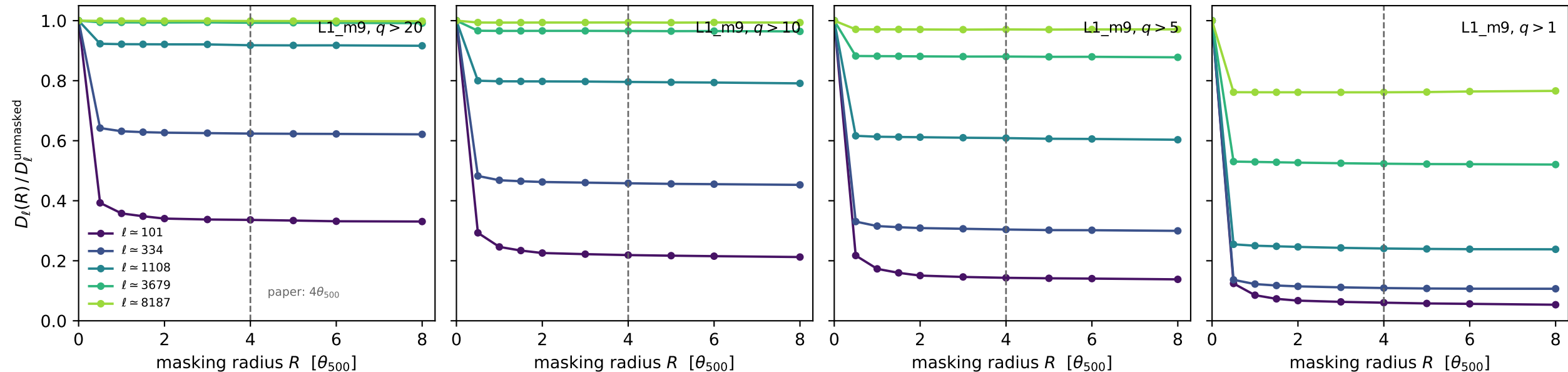
Masking-radius null test: surviving tSZ power
