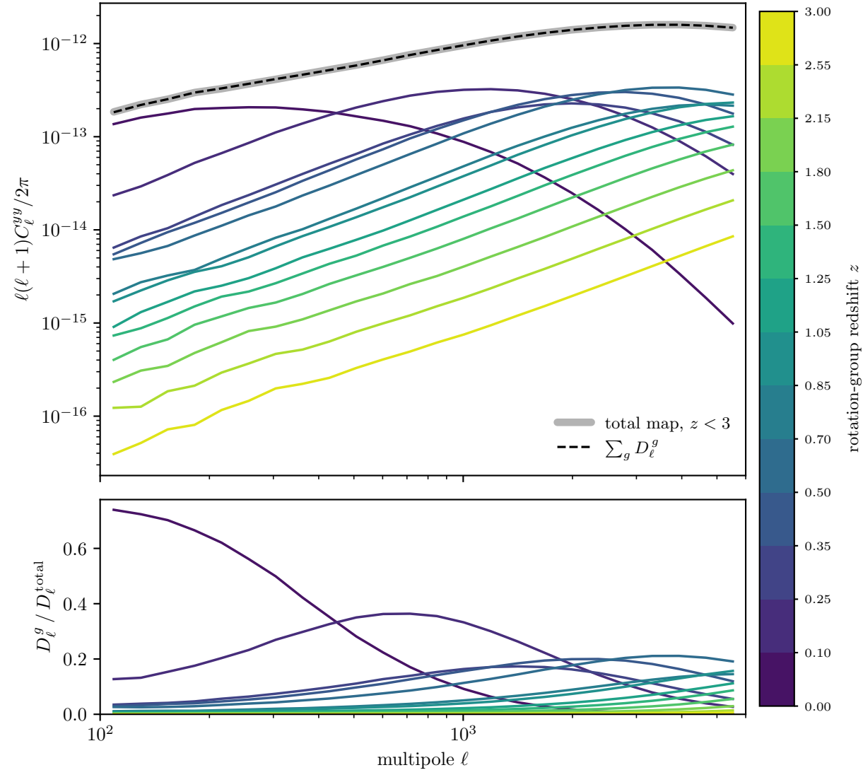
FLAMINGO L1_m9: the tSZ power spectrum by lightcone redshift shell
