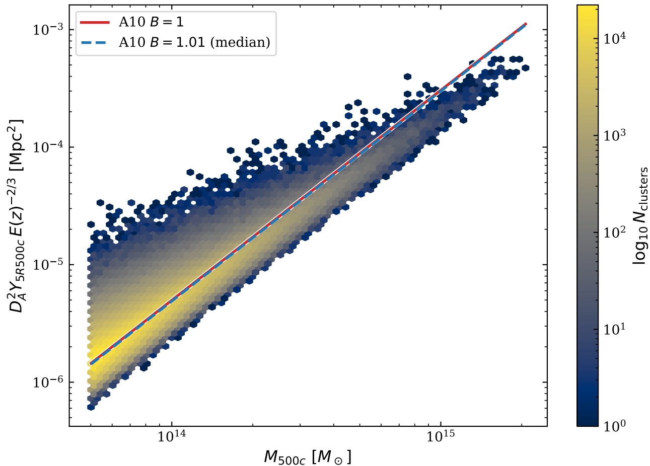
Y - M relation vs A10 (evaluated at z = 0.83 )
