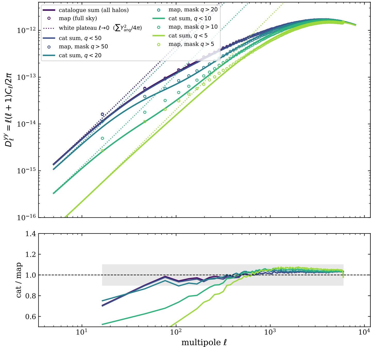
1-halo tSZ power spectrum: catalogue sum (GNFW, B = 1 ) vs map
