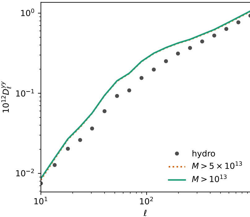
full sky
