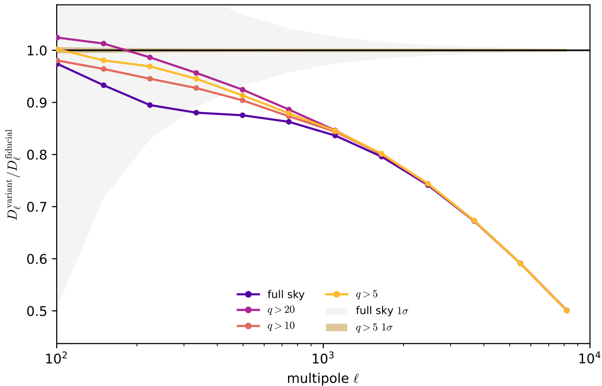
FLAMINGO L1_m9: f_{\text{gas}} - 8\sigma / fiducial ratio vs sky cut (12 log bins ( \Delta \ln \ell = 0.4 ); \alpha_{\text{SZ}} = 1.12 ; bands: full-sky and q > 5 theory 1\sigma about 1)
