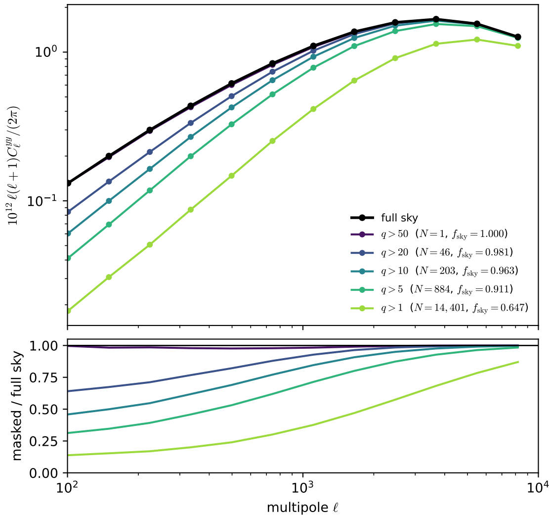
FLAMINGO L2p8_m9 fiducial (lc0): masked tSZ power spectrum ( \alpha_{\text{SZ}} = 1.12 best-fit q , \Delta \ln \ell = 0.4 log bins)
