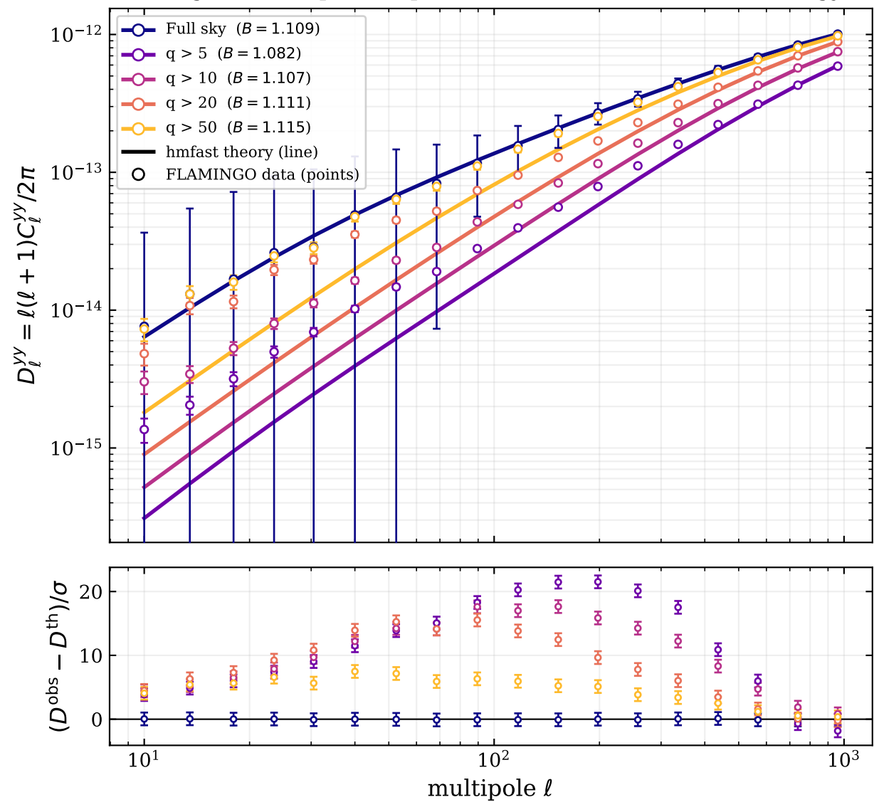
Pure-gNFW tSZ power spectrum at best-fit B (D3A cosmology)
