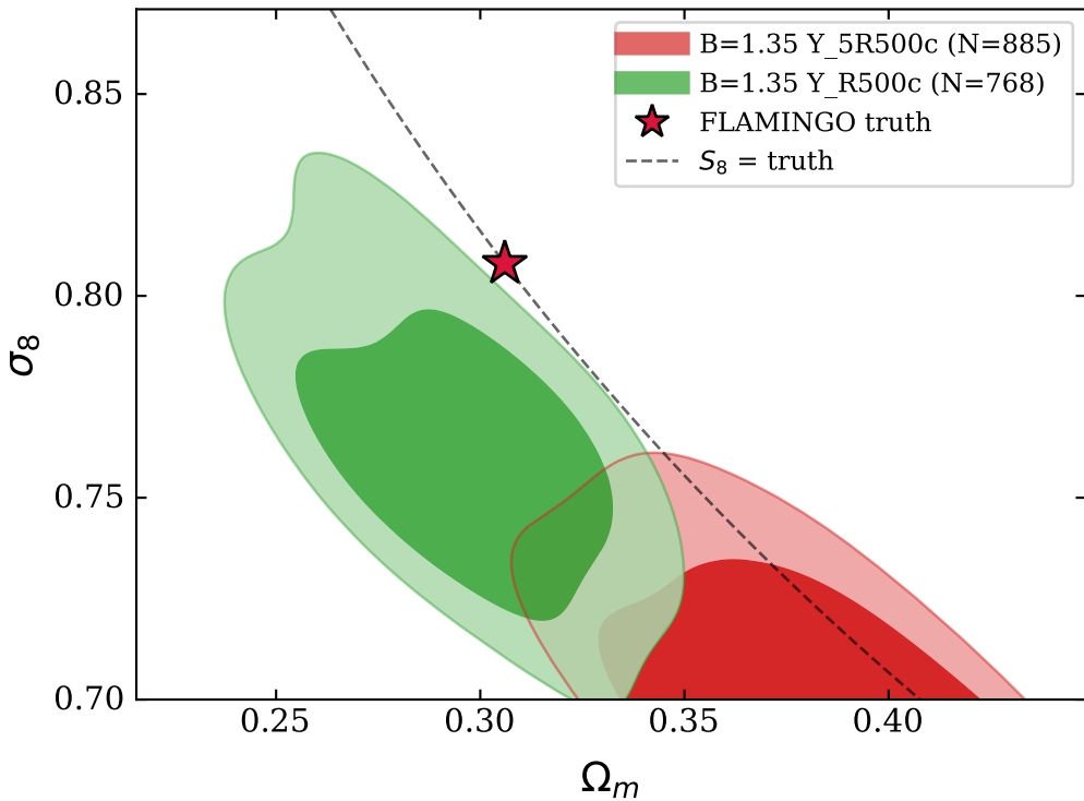
B=1.35: Y_{5R500c} vs Y_{R500c}
