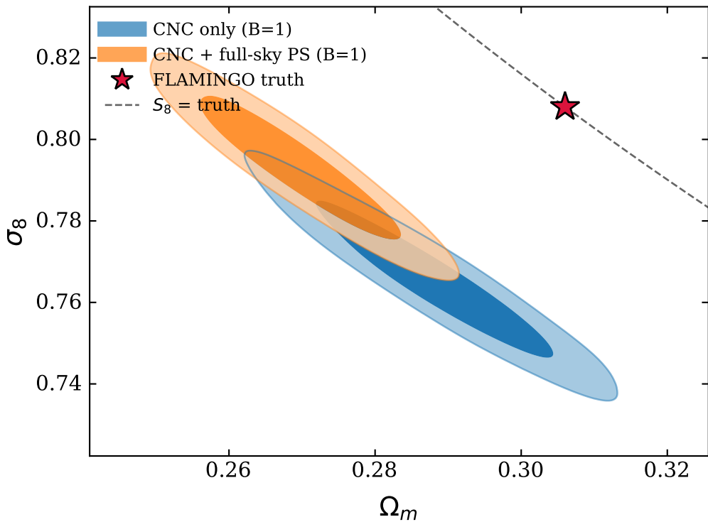
B=1 + fixOb: CNC vs CNC+full-sky tSZ PS
