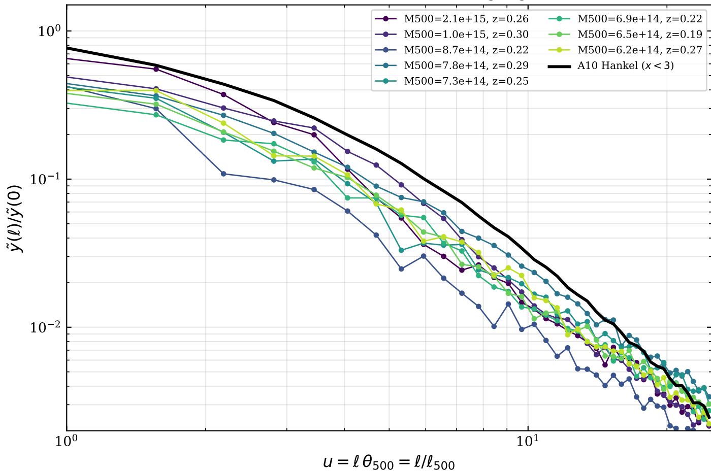
Per-cluster Fourier form factors (log-log scale)
