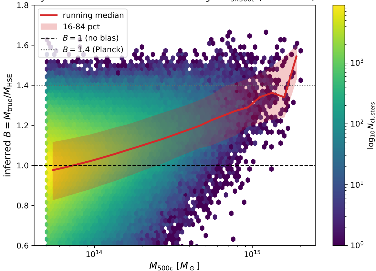
Hydrostatic bias inferred from catalogue Y_{5R500c} (A10 GNFW)
