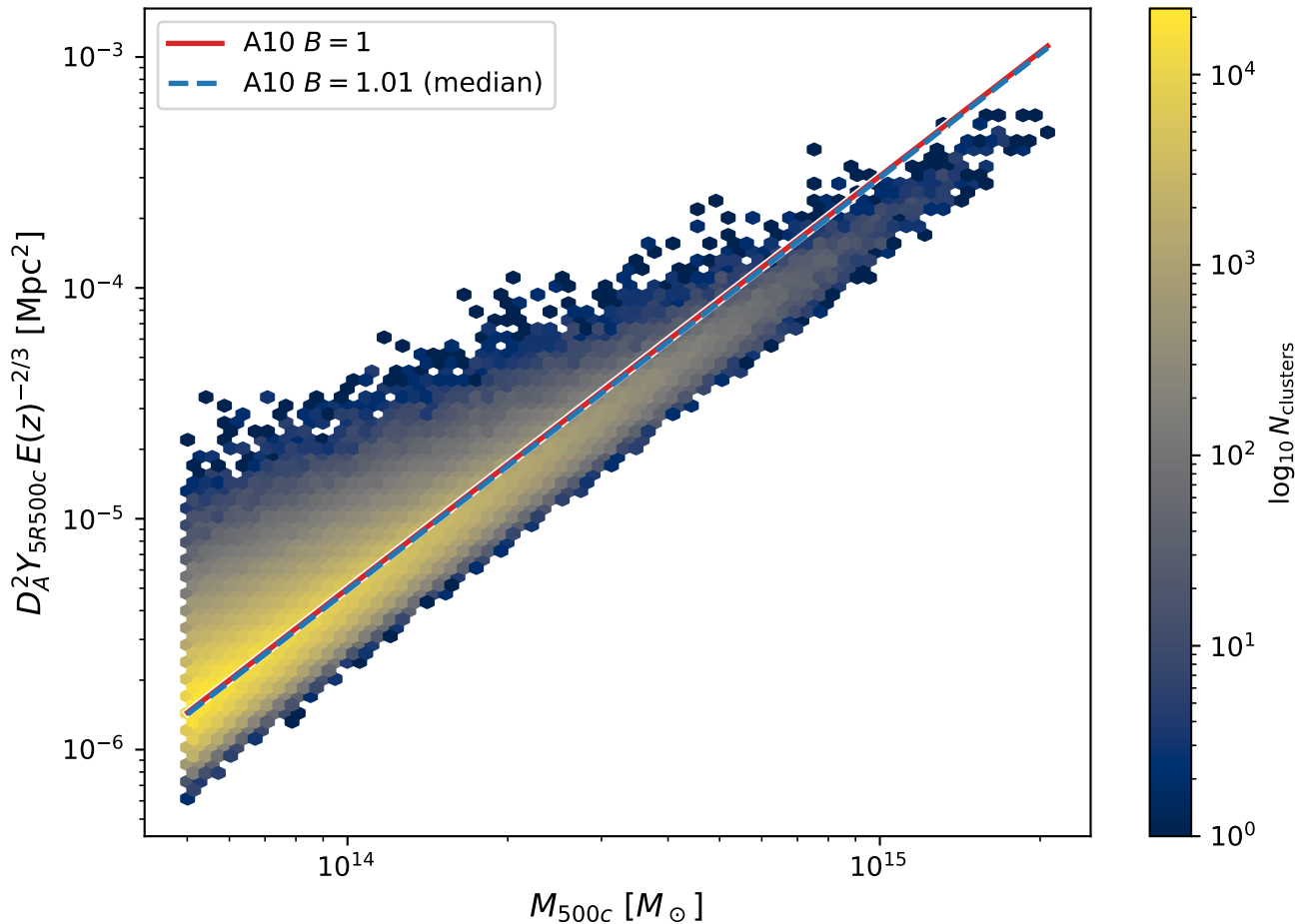
Y-M relation vs A10 (evaluated at z = 0.83 )
