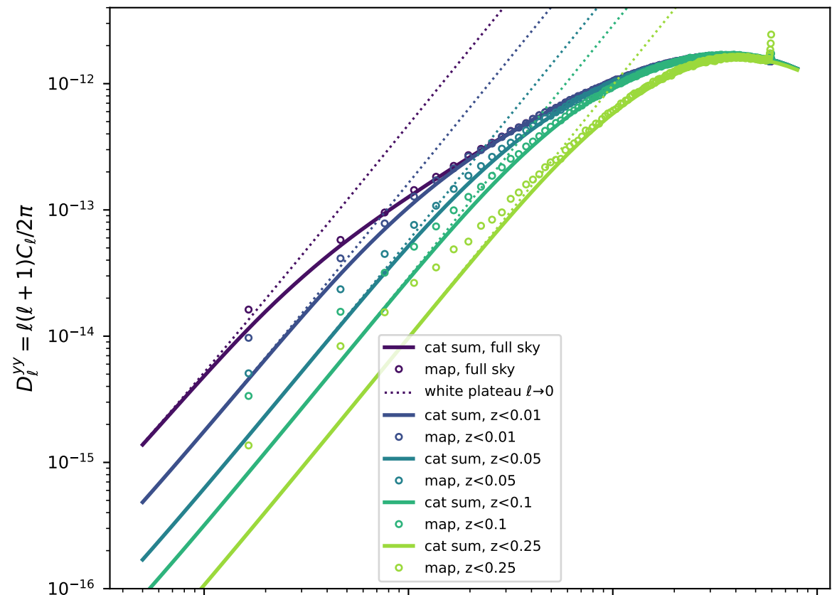
Mask low redshift: z < z_{\text{cut}}
