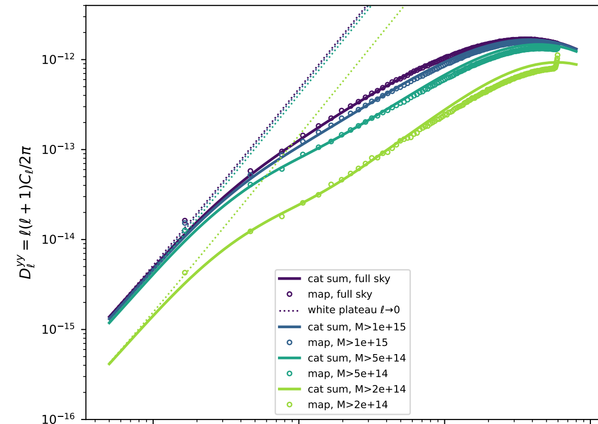
Mask high mass: M_{500c} > M_{\text{cut}}
