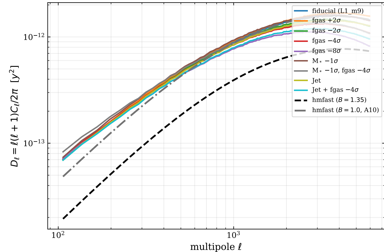
L1_m9 feedback: masked tSZ PS ( q > 20 , q_{\text{from\_mz}} > 20 )
