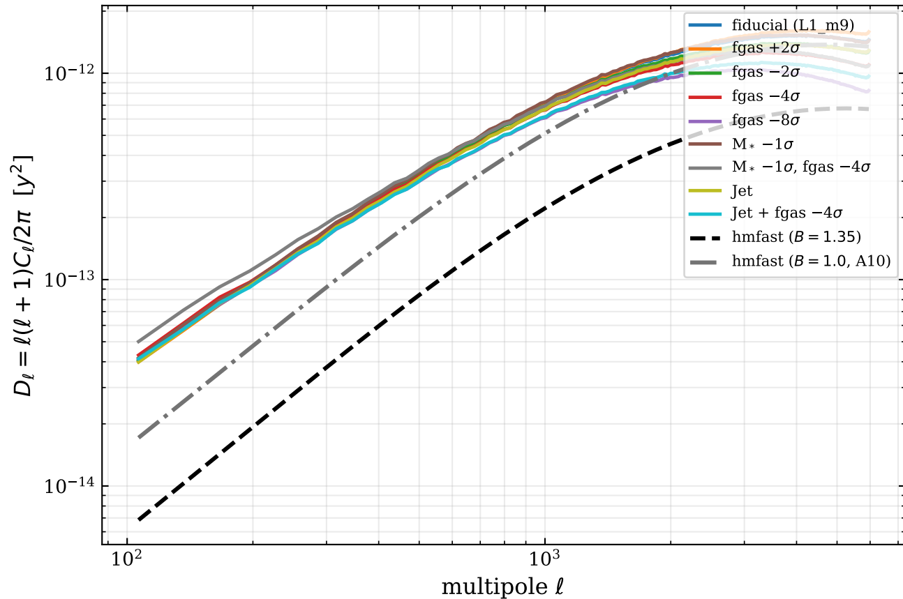
L1_m9 feedback: masked tSZ PS ( q > 5 , q_{\text{from\_mz}} > 5 )
