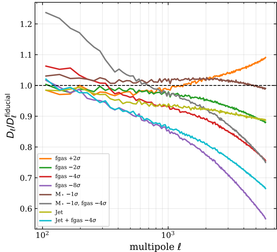
Masked q > 5 : ratio to fiducial L1_m9 ( q_{\text{from\_mz}} > 5 )
