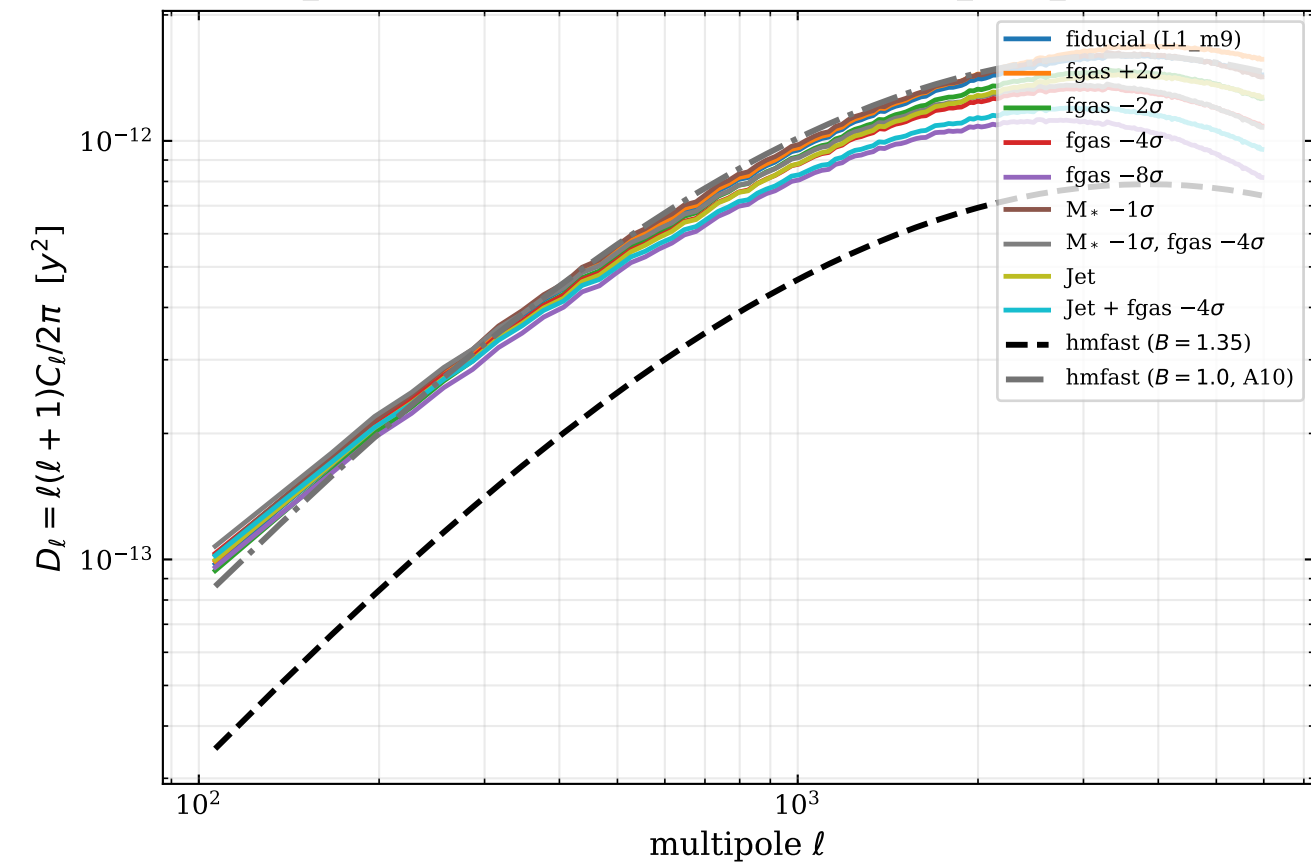
L1_m9 feedback: masked tSZ PS ( q > 50 , q_{\text{from\_mz}} > 50 )
