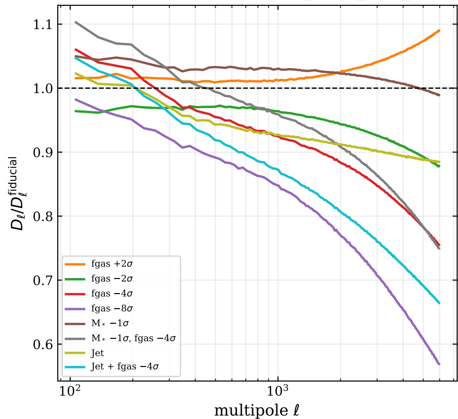
Masked q > 50 : ratio to fiducial L1_m9 ( q_{\text{from\_mz}} > 50 )
