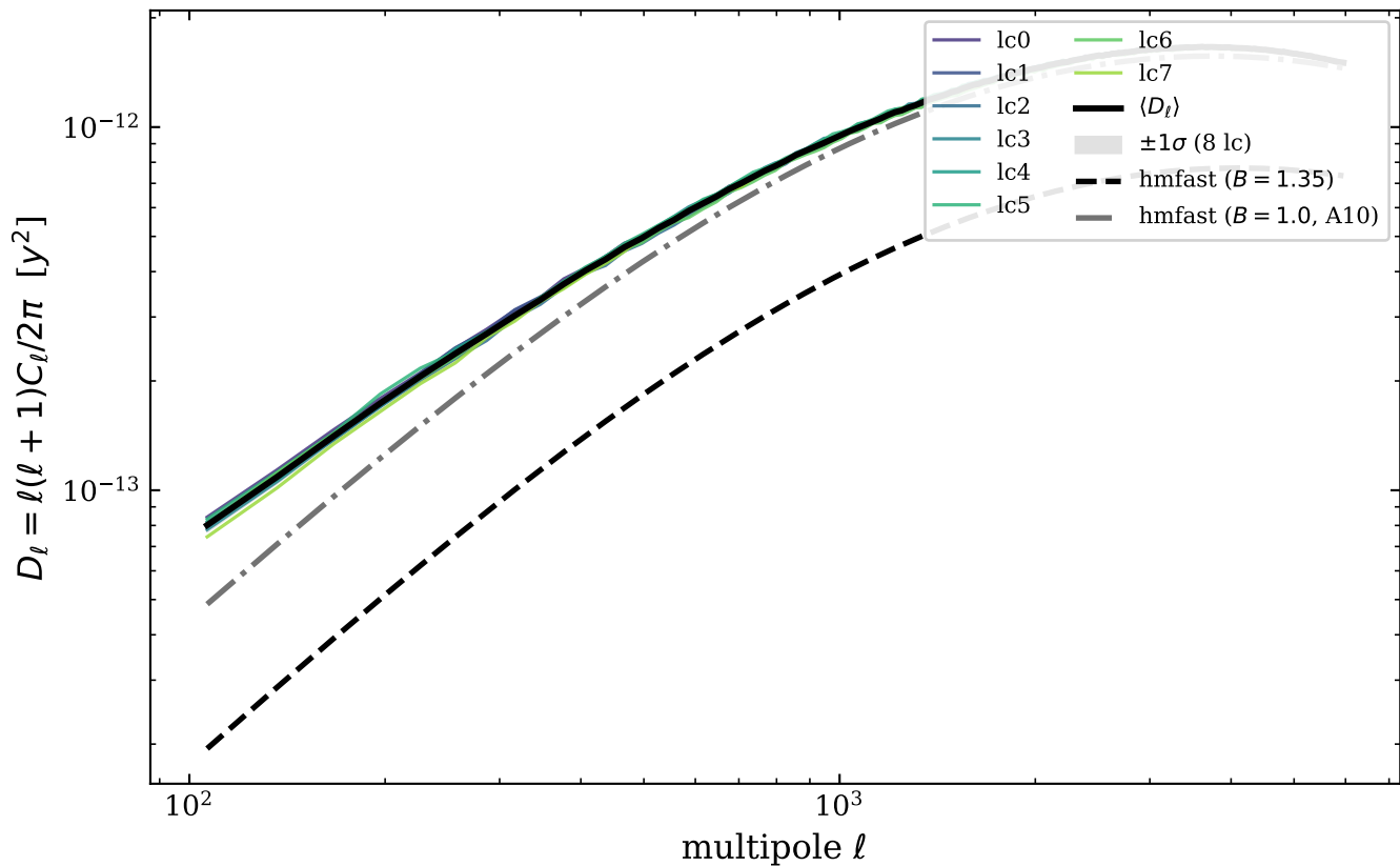
L2p8_m9 masked tSZ PS — q > 20
