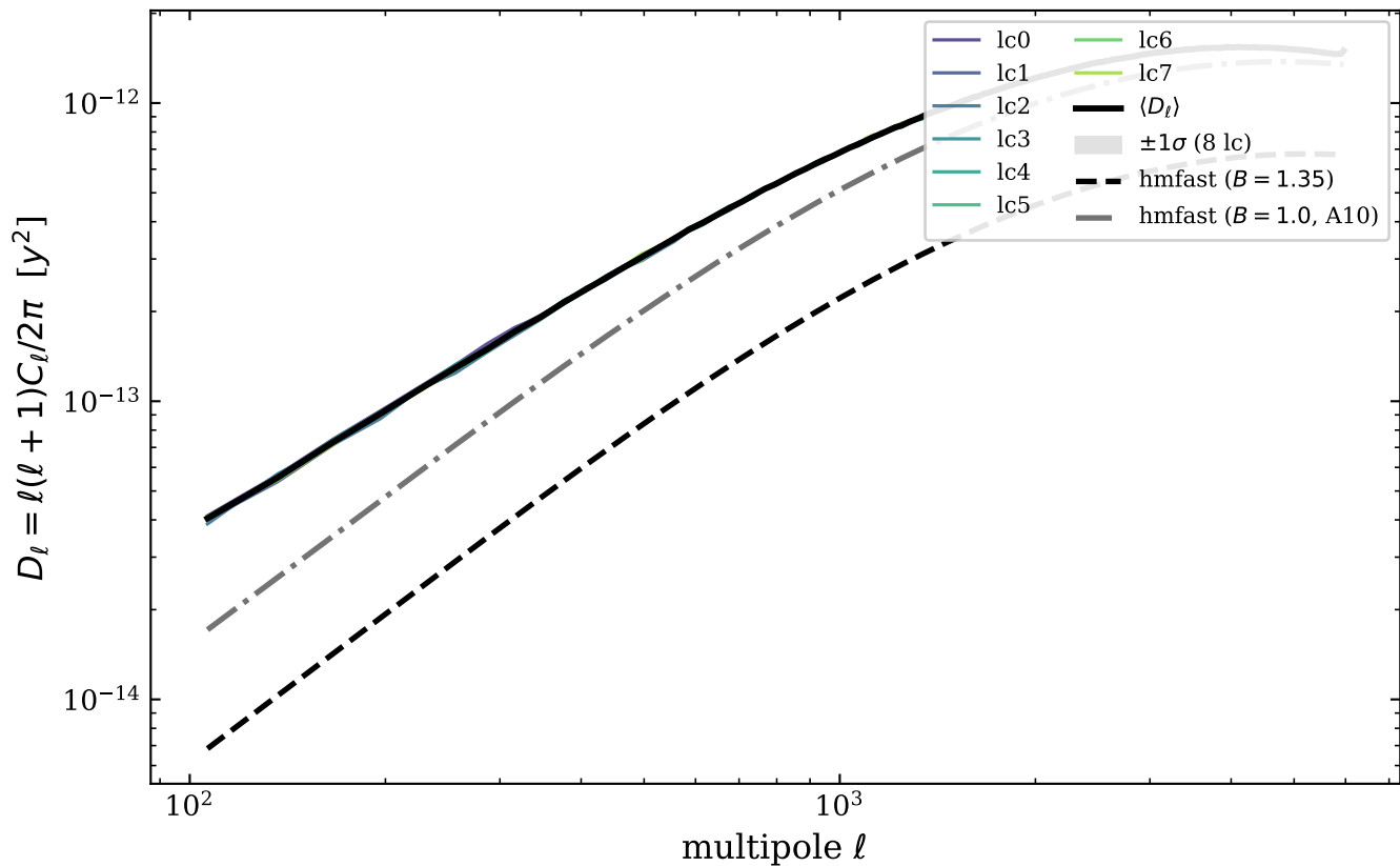
L2p8_m9 masked tSZ PS — q > 5
