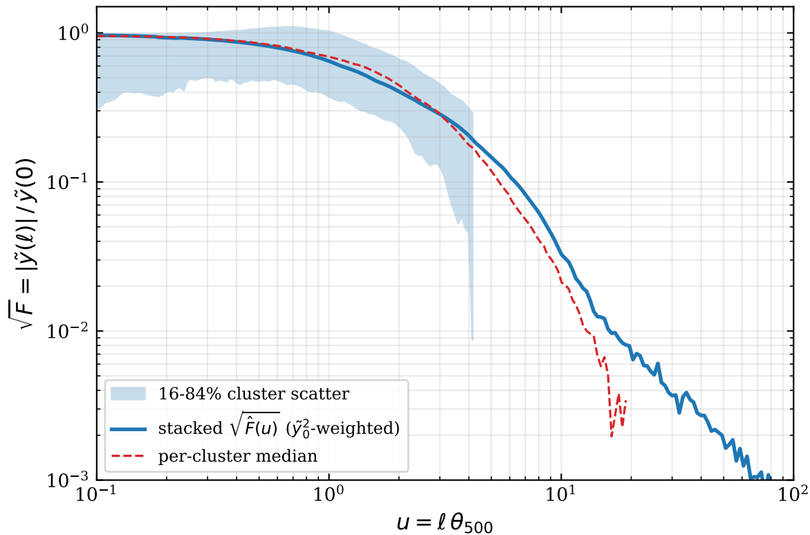
Fourier-space stacked profile: 1088 clusters ( q > 5 , aperture 5 \theta_{500} )
