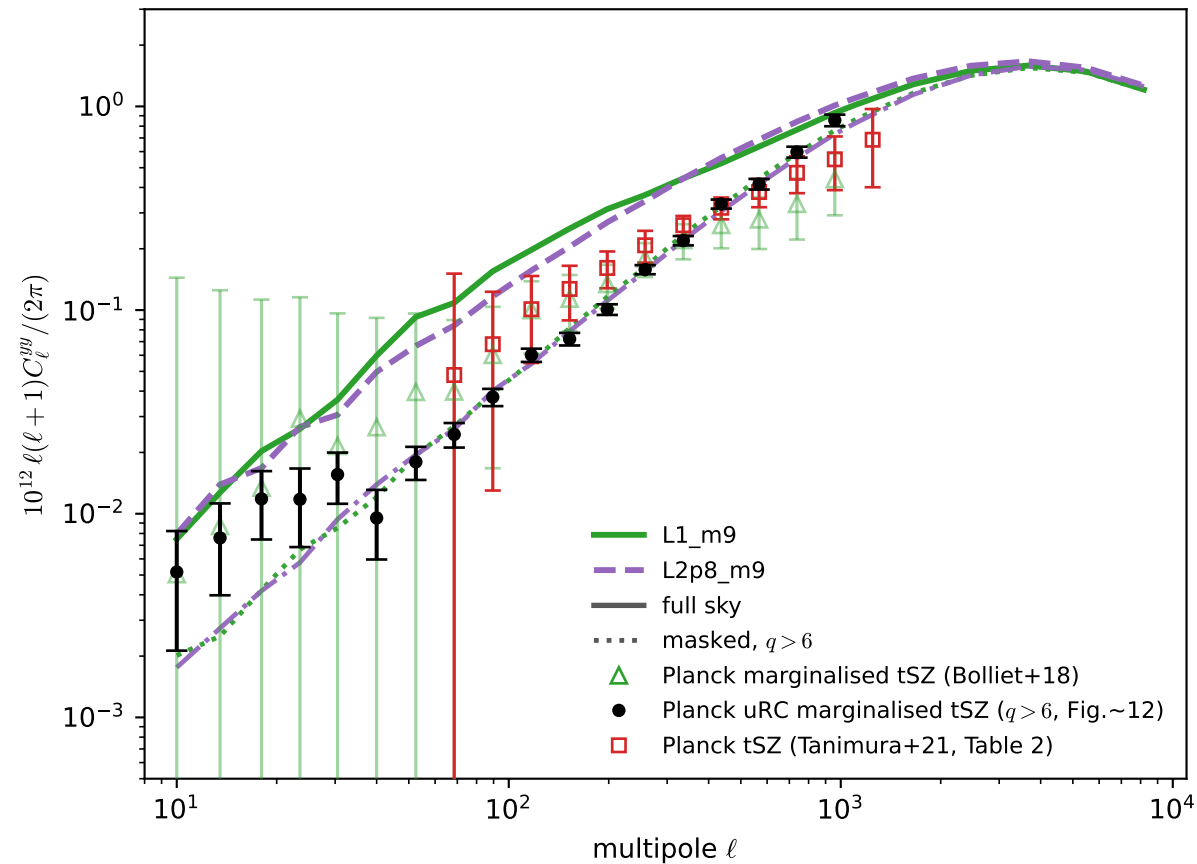
FLAMINGO fiducial tSZ vs Planck ( \alpha_{\text{SZ}} = 1.12 best-fit q )
