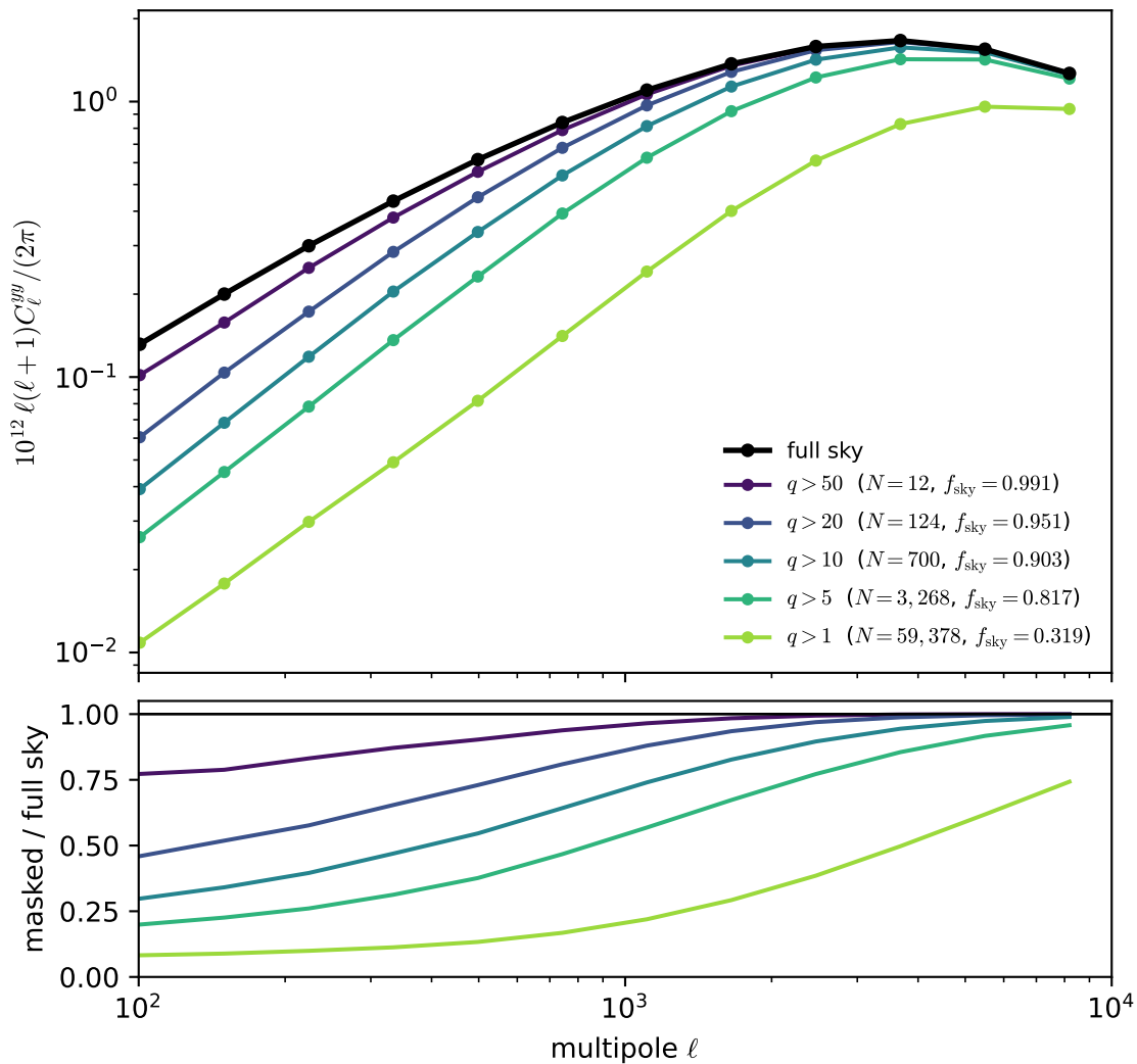
FLAMINGO L2p8_m9 fiducial (lc0): masked tSZ power spectrum (empirical aperture q , \Delta \ln \ell = 0.4 log bins)
