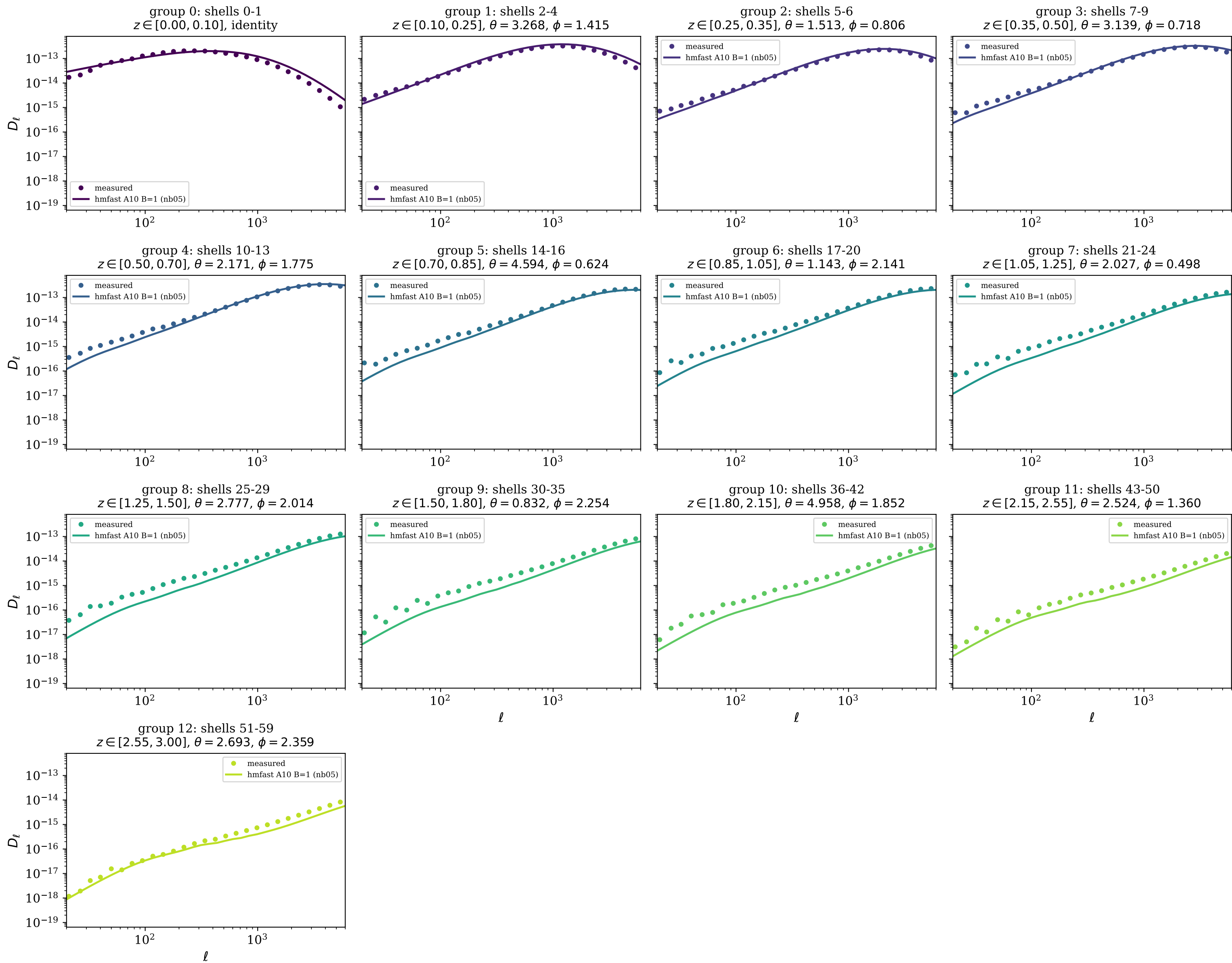
L1_m9 lc0 (fiducial): tSZ D_\ell per rotation-group shell sum vs hmfast (A10 GNFW, B = 1.0 )
