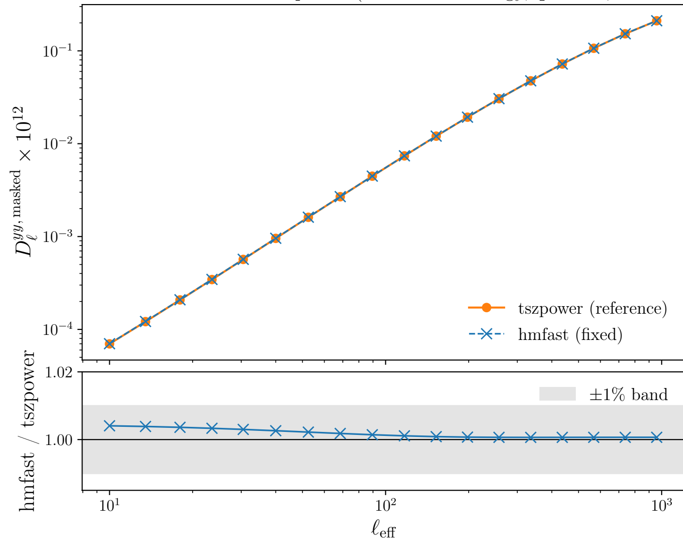
Masked tSZ D_\ell : hmfast vs tszpower (fiducial cosmology, q_{\text{cat}} = 5 , \sigma_{\ln Y} = 0.173 )
