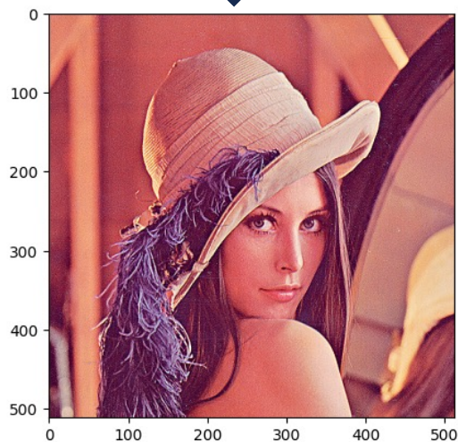
Sharpen kernel
