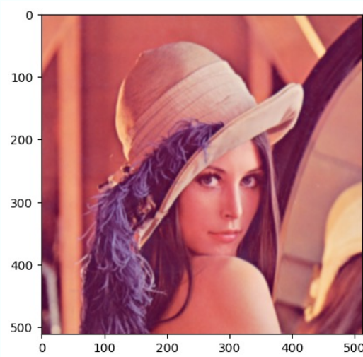
Gaussian kernel
