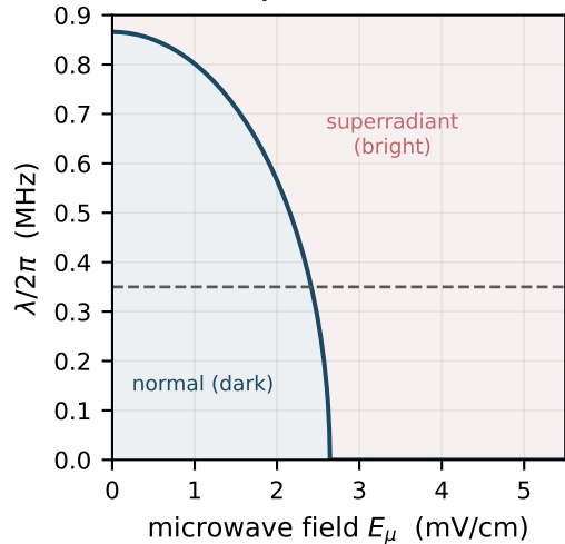
(a) boundary at fixed \delta : field turns it ON
