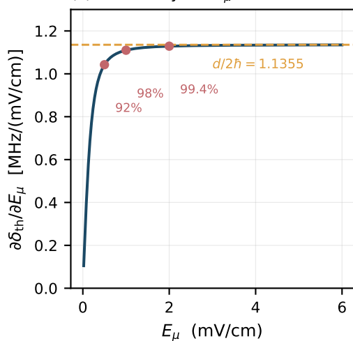
(c) linear only for \Omega_\mu \gg 2\lambda^2/\omega
