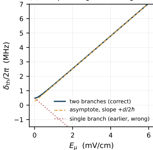
(b) lock point: sign was wrong
