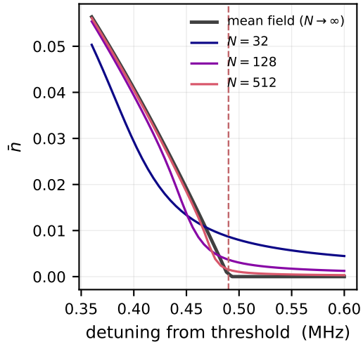
(b) finite- N rounding, \propto N^{-2/3}
