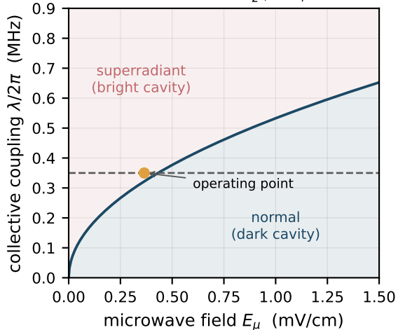
(a) threshold line \lambda_c = \frac{1}{2}\sqrt{\omega \Omega_\mu/2}
