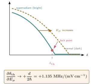
(c) what the servo locks to
