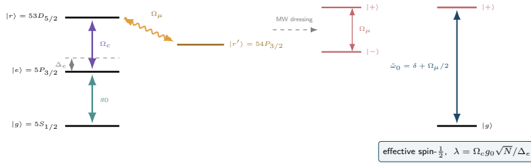
(b) level scheme
