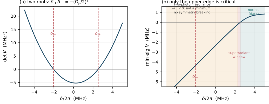
Figure 3: Two roots, one critical point ( \omega/2\pi = 1 MHz, \lambda/2\pi = 0.35 MHz, E_\mu = 2 mV/cm, so \Omega_\mu/2 = 2\pi \times 2.271 MHz). (a) \det V is an upward parabola in \delta with roots \delta_- = -2.039 and \delta_+ = +2.529 MHz/ 2\pi , obeying \delta_+ \delta_- = -\Omega_\mu^2/4 . (b) The smallest eigenvalue of V , however, crosses zero only at \delta_+ . Below \delta = \Omega_\mu/2 the normal phase is already not a minimum because \omega_- < 0 , so \delta_- marks no transition. The asymmetry is one of accessibility, not of physics: written in the near-resonant splitting, both sides have the same threshold |\omega_{\text{near}}| = 2\lambda^2/\omega .
