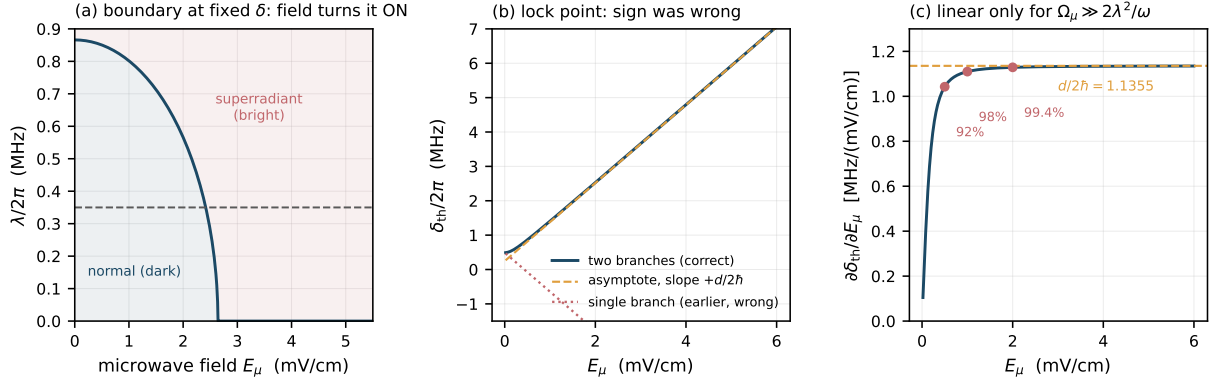
Figure 2: The microwave field moves the phase boundary — corrected for both dressed branches. \omega/2\pi = 1 MHz, \lambda/2\pi = 0.35 MHz, \delta/2\pi = 3 MHz. (a) The boundary Eq. (17) at fixed \delta : \lambda_c falls with the field, so raising E_\mu switches the cavity on. (b) The Protocol B lock point. The correct two-branch result (solid) rises with slope +d/2\hbar ; the single-branch model of earlier drafts (dotted) falls with slope -d/2\hbar — the same magnitude and the wrong sign. (c) The scale factor reaches d/2\hbar only asymptotically, hitting 92% at 0.5 mV/cm, 98% at 1 mV/cm and 99.4% at 2 mV/cm, and vanishing as E_\mu \rightarrow 0 .
