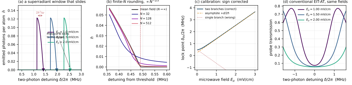
Figure 5: The Protocol B read-out, computed ( \omega/2\pi = 1 MHz, \lambda/2\pi = 0.35 MHz). (a) Emitted photons per atom versus two-photon detuning. With both dressed branches kept, the superradiant region is a window of field-independent width 2\lambda^2/\omega that slides rigidly at +1.135 MHz per (mV/cm); Protocol B locks to the upper edge. (b) Finite- N rounding, \propto N^{-2/3} — computed in the single-branch model, where exact diagonalisation is cheap, but the scaling law is universal for this class and carries over. (c) The corrected calibration (solid), its asymptote +d/2\hbar (dashed), and the single-branch result of earlier drafts (dotted), which has the wrong sign. (d) Conventional EIT-AT transmission at the same fields, for contrast. It responds well; the difference between the two read-outs is the shape of the discriminant, not that one of them fails.
