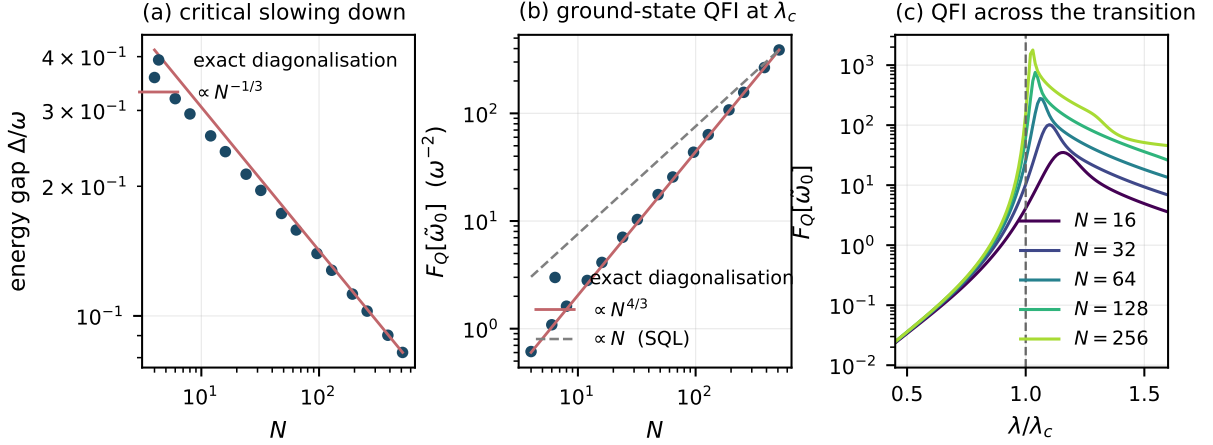
Figure 6: Finite-size scaling at the critical point ( \omega = \tilde{\omega}_0 = 1 , \lambda = \lambda_c , N \leq 512 ). (a) The energy gap closes as N^{-1/3} (fitted -0.317 over N \geq 128 ). (b) The quantum Fisher information for \tilde{\omega}_0 grows as N^{4/3} (fitted 1.307 over N \geq 128 ), super-extensive and thus formally beyond the standard quantum limit F_Q \propto N (dashed). (c) F_Q across the transition; the peak sharpens and moves towards \lambda_c as N grows.
