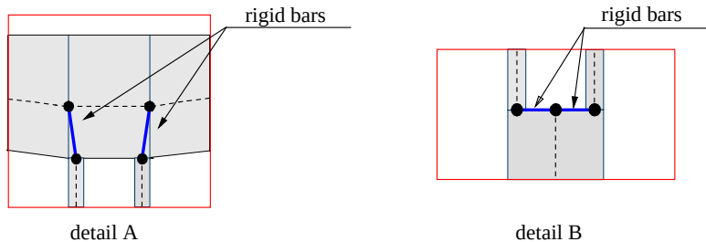
b) Details of the rigid bars
