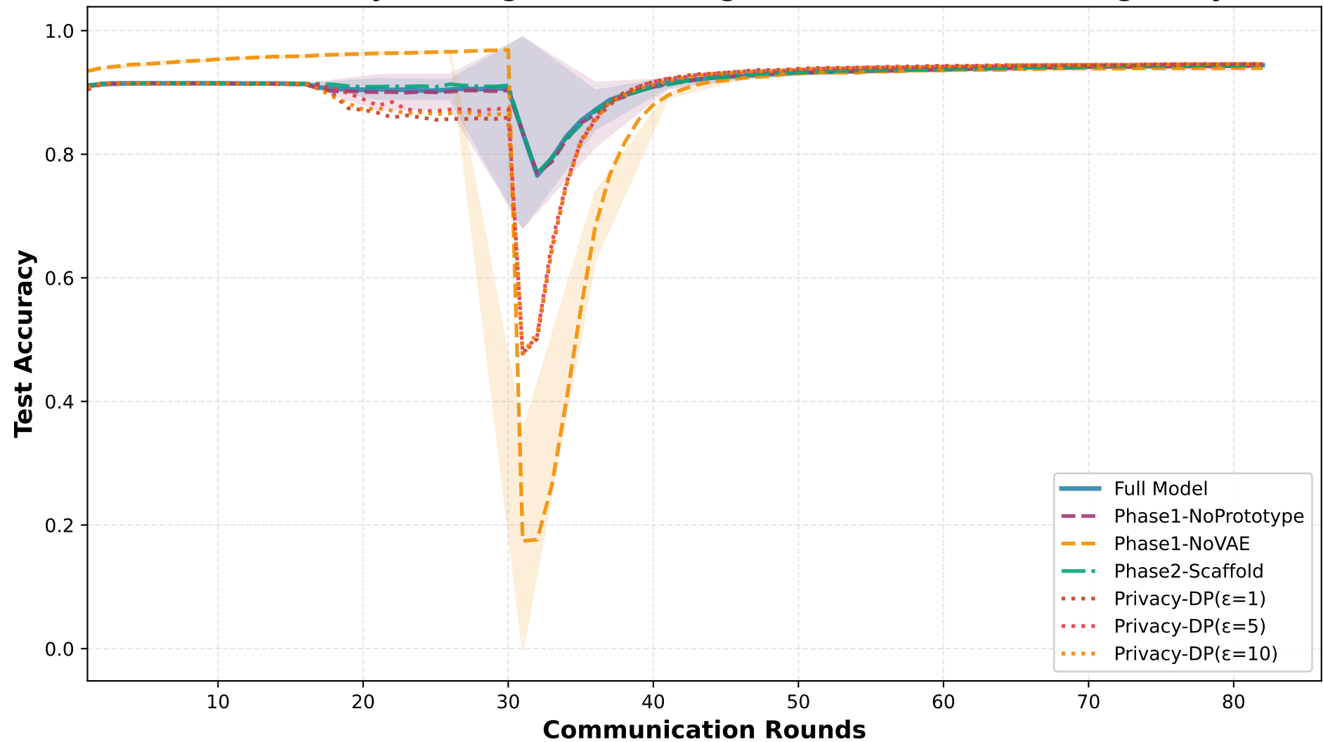
Ablation Study Convergence (Xinwang Dataset - Feature Heterogeneity)
