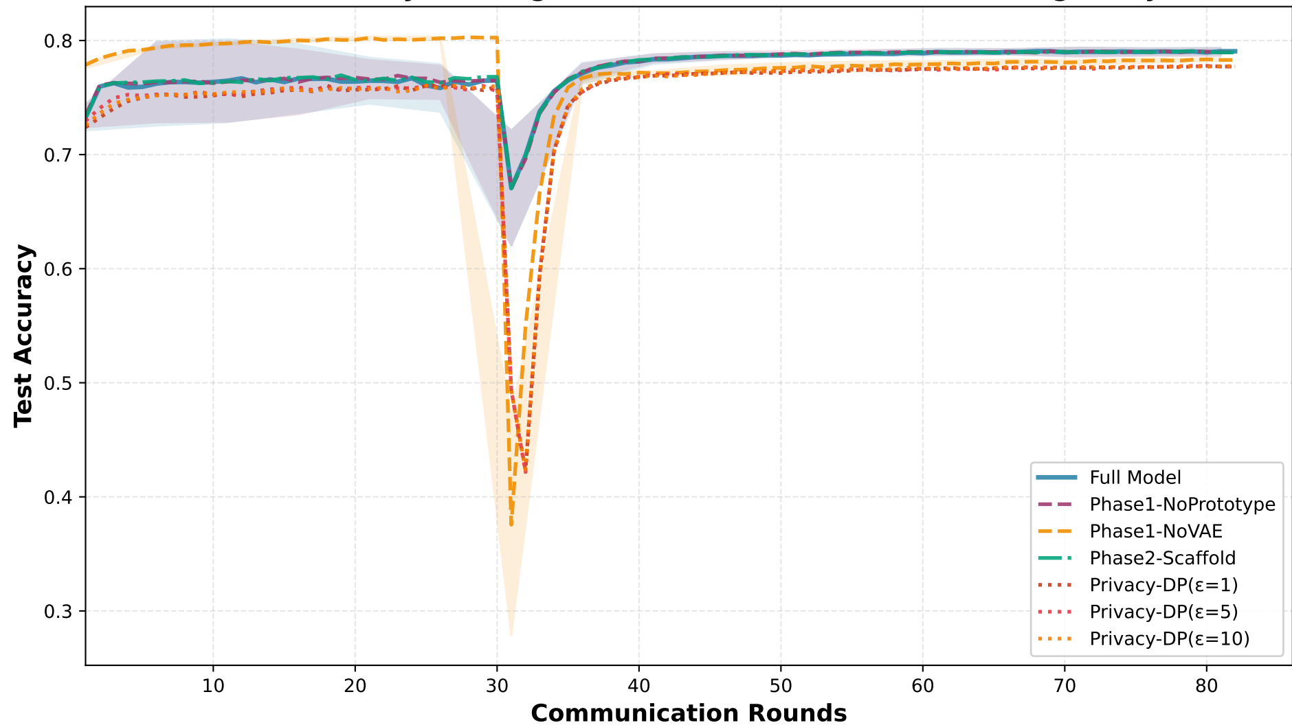
Ablation Study Convergence (Uci Dataset - Feature Heterogeneity)
