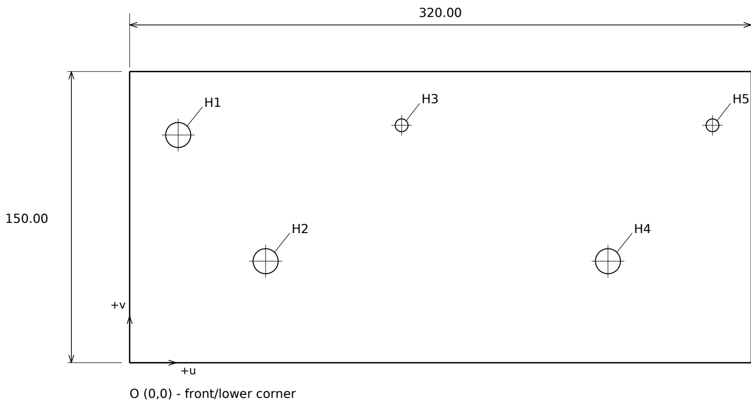
PRINCIPAL VIEW - looking along -X THIRD-ANGLE ORTHOGRAPHIC PROJECTION | SCALE 1:2
