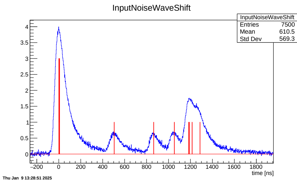
Figure 1: Simulated data convoluted with Landau SIPM resolution
