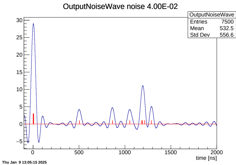
Figure 2: Wiener deconvoluted output with input photon distribution
