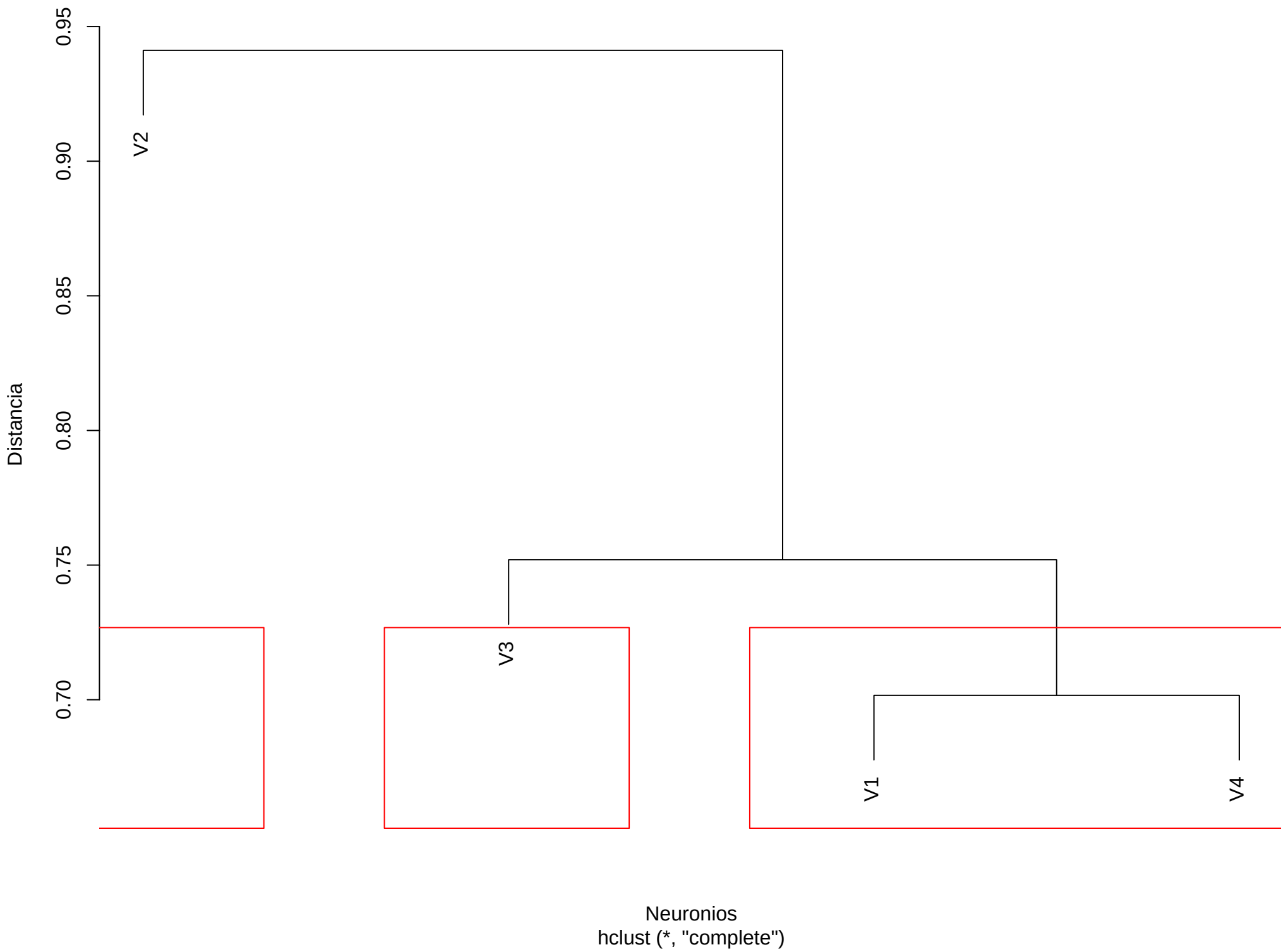
Dendrograma (k=3) | scene | gaussian | Fold 1
