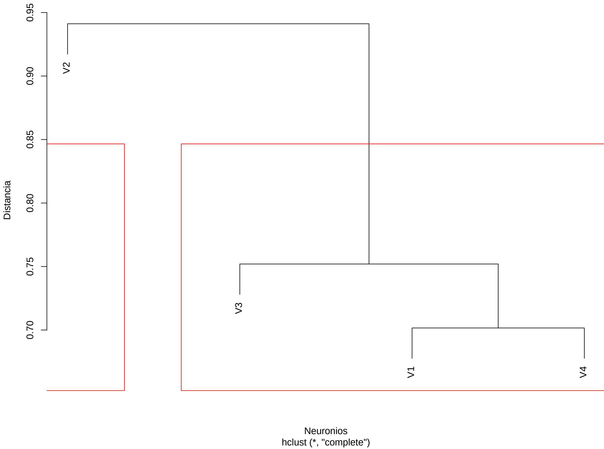
Dendrograma (k=2) | scene | gaussian | Fold 1
