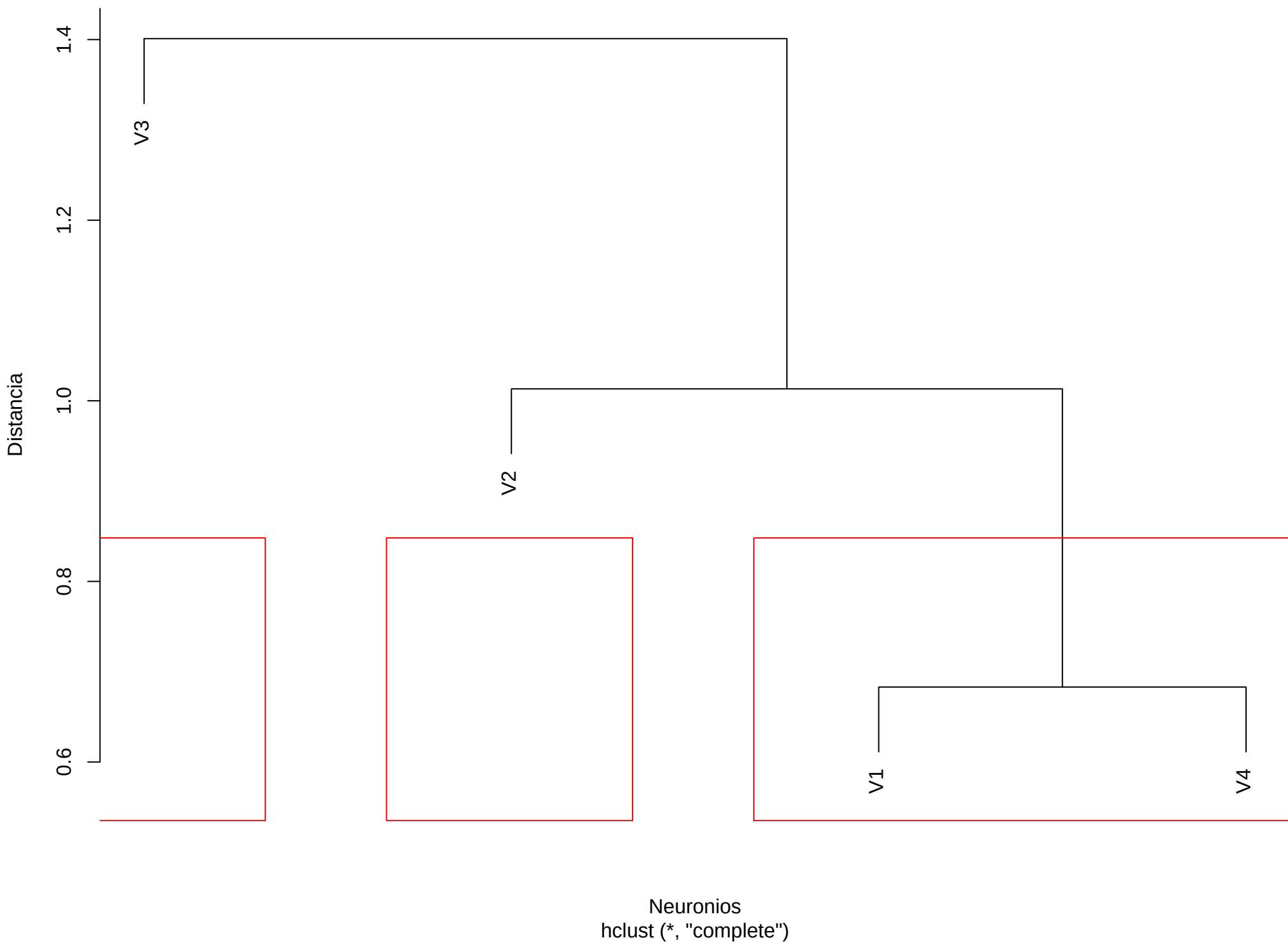
Dendrograma (k=3) | emotions | gaussian | Fold 3
